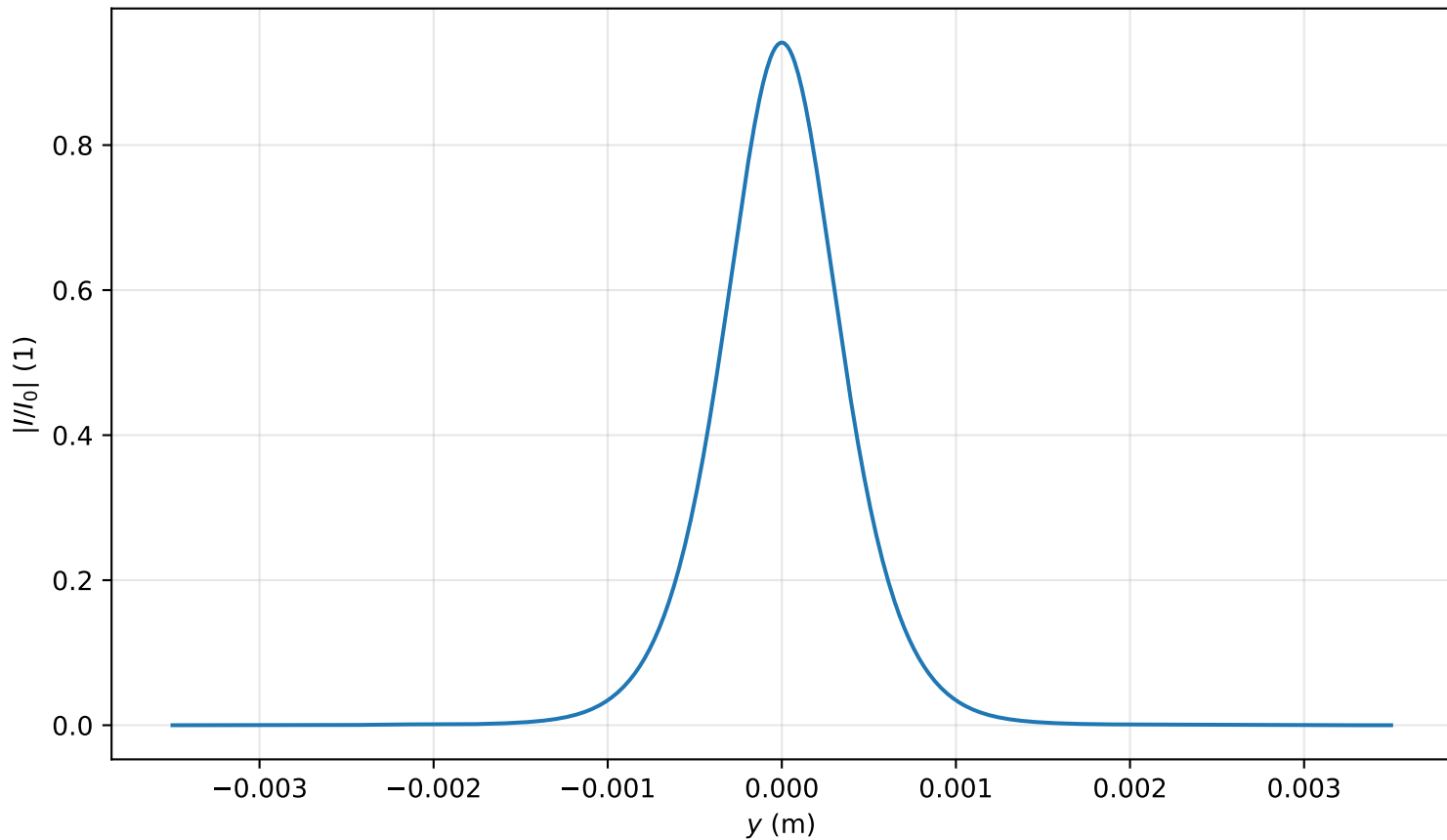
Intensity profile I(x=0, y, z=3.662)/I_0 , P_{in}=0.8P_{cr} , artificial time
